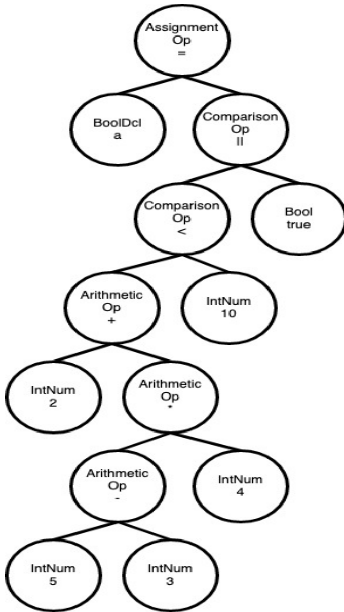
Figure 3: AST before constant folding
