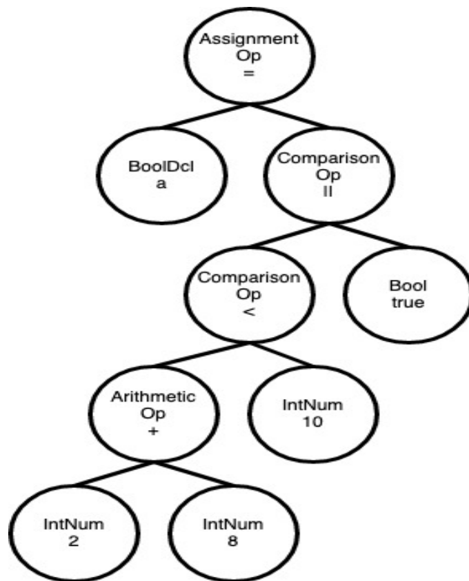
Figure 5: Constant folding: step 2
